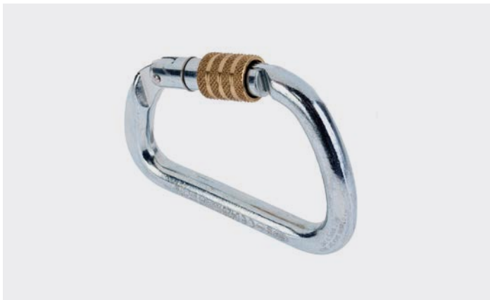
HR031 Carabiner - 45kN
