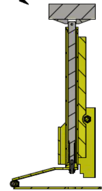
SECTION A-A (1:10)
