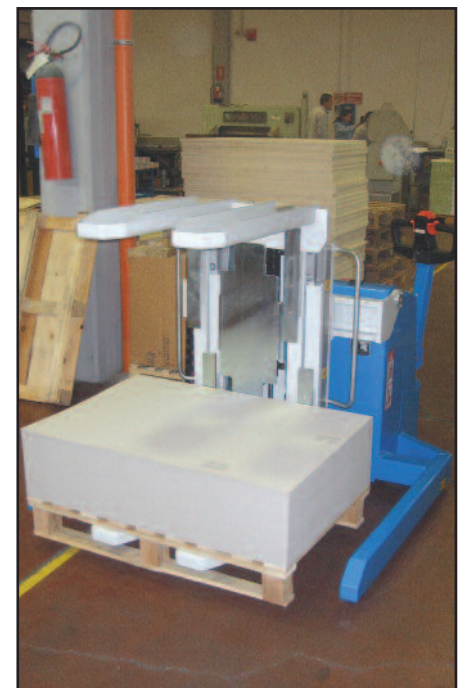
Argo M10AS straddle version for double faced pallets
