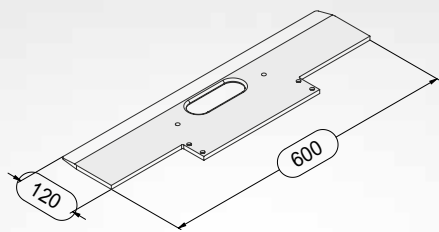
Toe plate 600 x 120 mm
