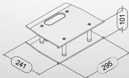
Toe plate for a laundry cart 295 x 241 x 101 mm
